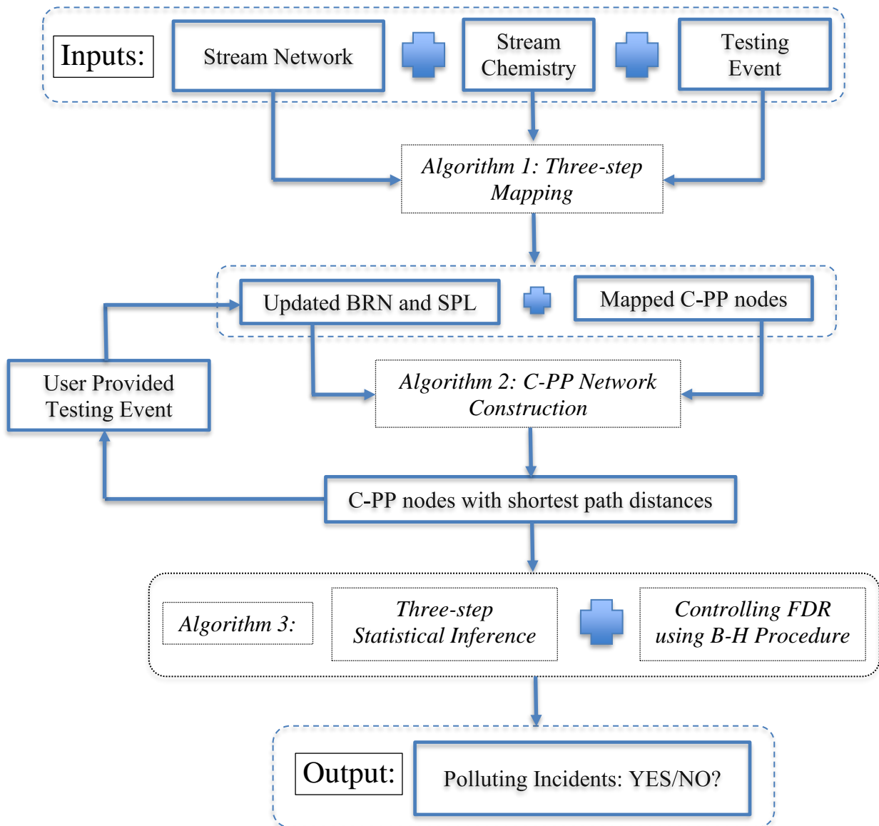
Figure 1. A flow chart illustrating the GeoNet Framework.
